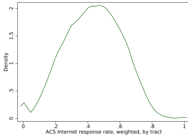
Figure 4: Kernel-smoothed probability distribution function of tract-level ACS Internet response rate, ACS, 2021 5-year file
