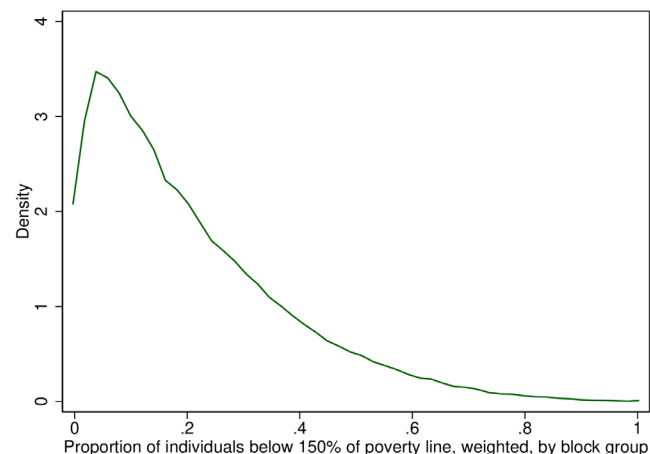
Figure 5: Kernel-smoothed probability distribution function of block-group-level 150% poverty rate, ACS, 2021 5-year file
