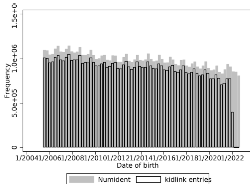
Figure 2. Frequency distributions of date of birth, Numident vs. CHCK entries, aged 0–17 years as of June 1, 2023
