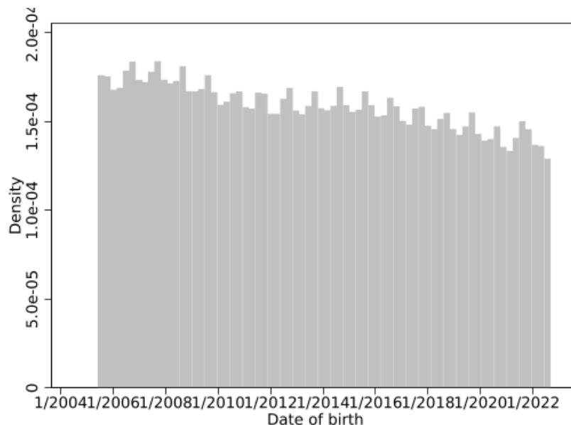
Figure 1: Distribution of date of birth, aged 0–17 years as of June 1, 2023, Numident
