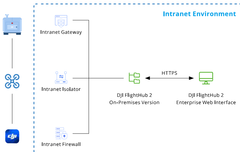
Figure 16 DJI FlightHub 2 On-Premises Version
