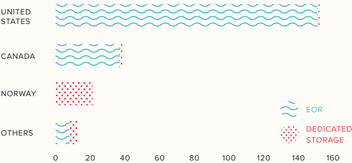
CUMULATIVE CO 2 INJECTION IN LEADING COUNTRIES 220 MILLION TONNES CO 2 INJECTED UNDERGROUND (APPROXIMATE VALUES)
