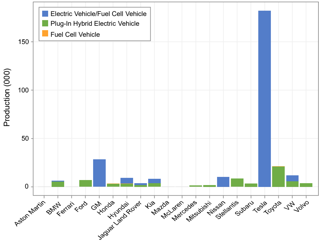
Figure 5.4. Model Year 2020 Production of EVs, PHEVs, and FCVs
